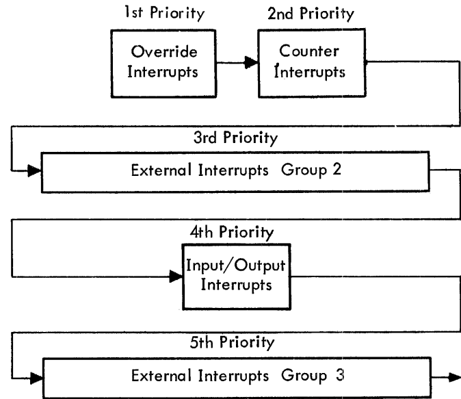
Figure 6. Typical Interrupt Priority Chain
