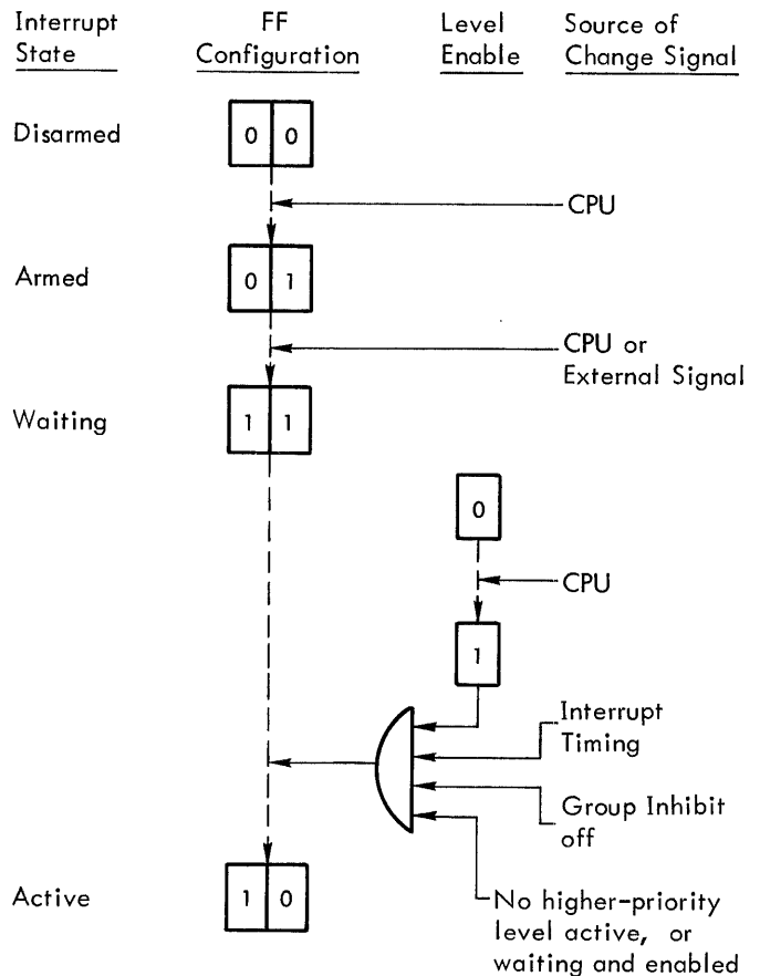
Figure 7. Interrupt Level Operation
