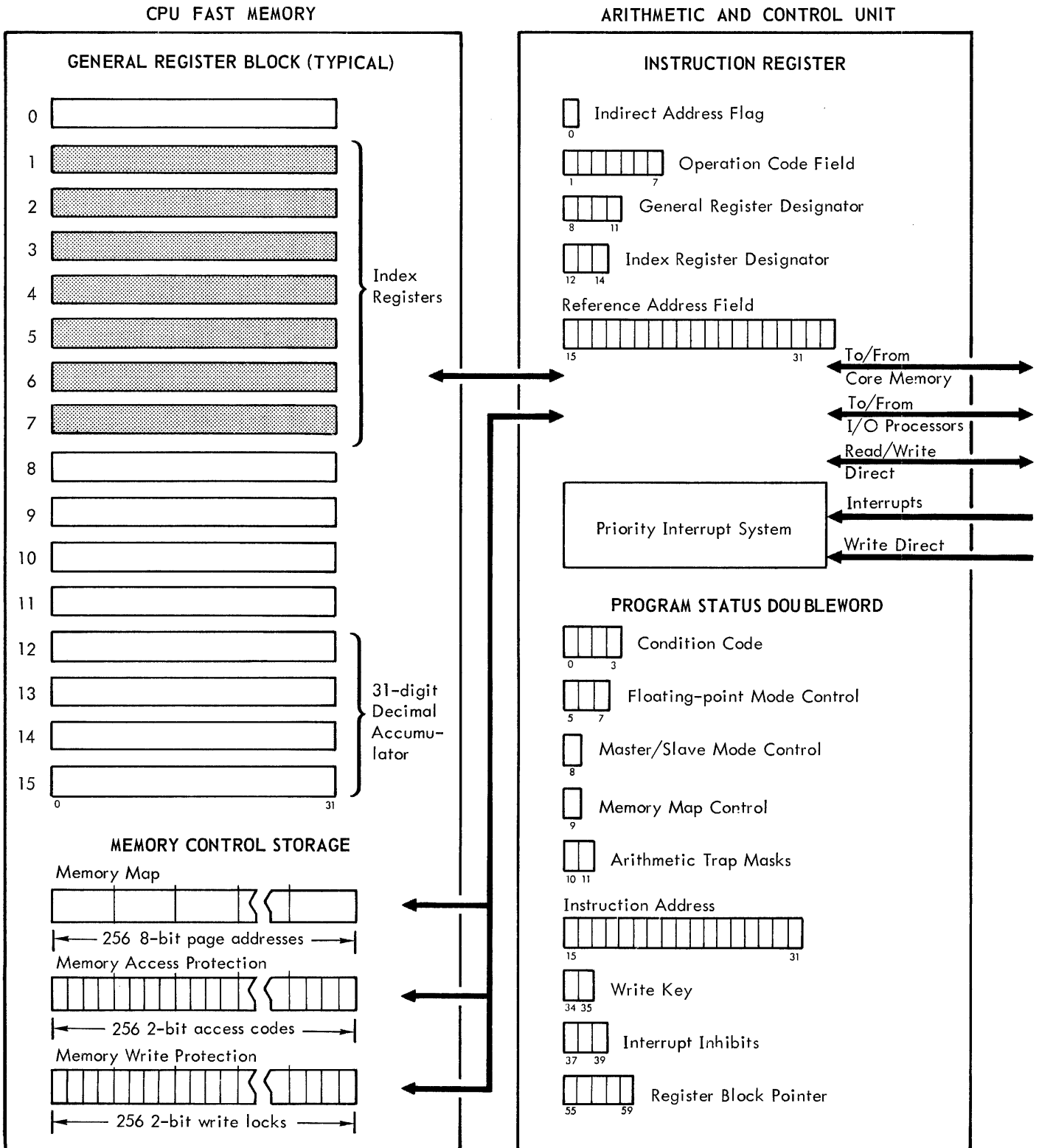
Figure 3. SIGMA 7 Central Processing Unit
