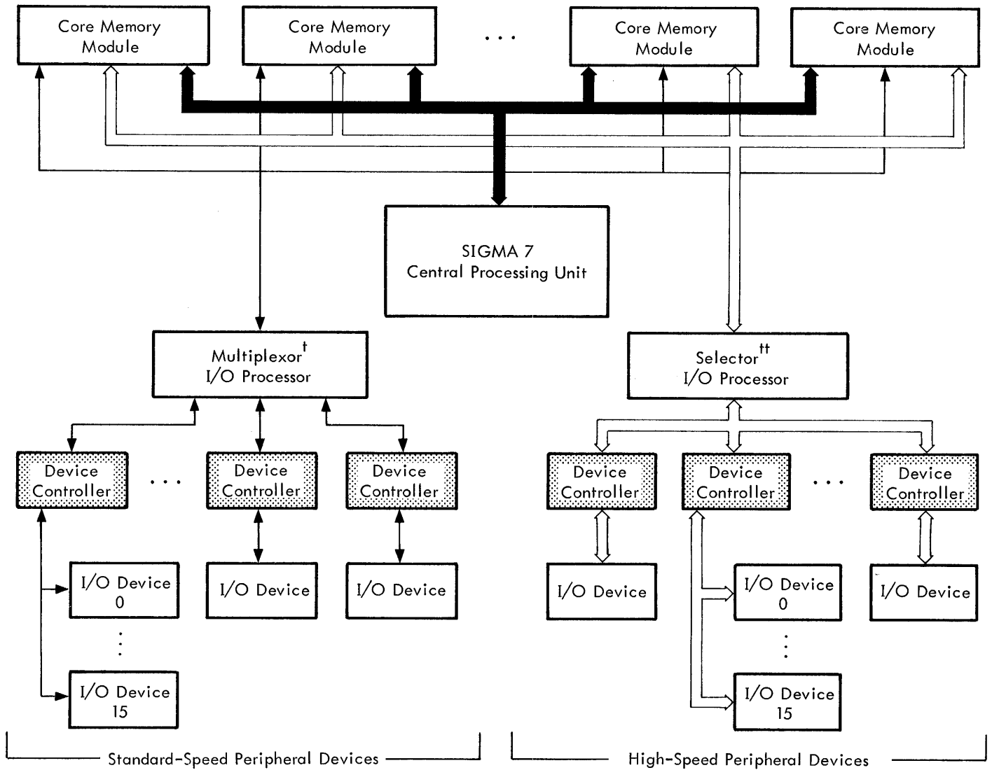
Figure 1. A Typical SIGMA 7 System
