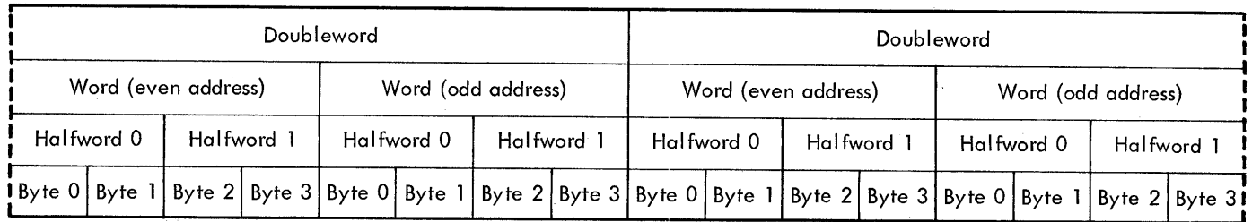
Figure 2. Information Boundaries
